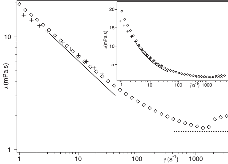
FIG. 9. Log-Log plot of the dynamic viscosity \mu of a 250 ppm scleroglucan solution at 23.6 °C as a function of \dot{\gamma} : (+) Low shear 30 rheometer; \diamond : Anton Paar MCR501 rheometer with double gap assembly. Solid and dotted lines: rheological laws using fitted parameter values listed in Table 2. Inset: lin-log plot of the same data.
