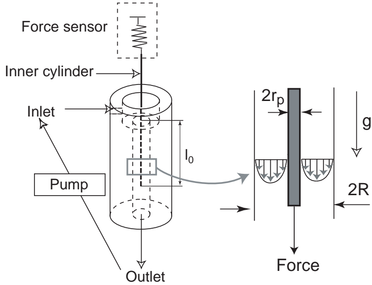
FIG. 1. Schematic view of the experimental viscometer.
