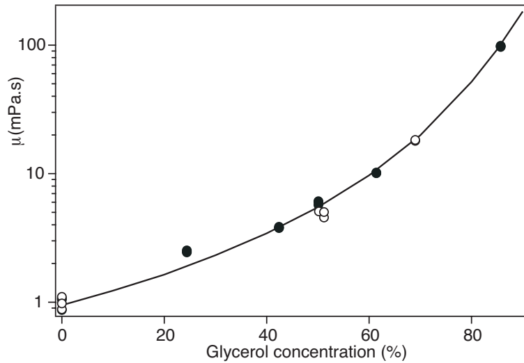
FIG. 7. Variation of the dynamic viscosity \mu as a function of the relative mass concentration of glycerol for water-glycerol solutions. Values obtained using ( \bullet ): device A ; ( \circ ): device B . Solid line: values from Ref. 17 for T = 22.6^\circ\text{C} .
