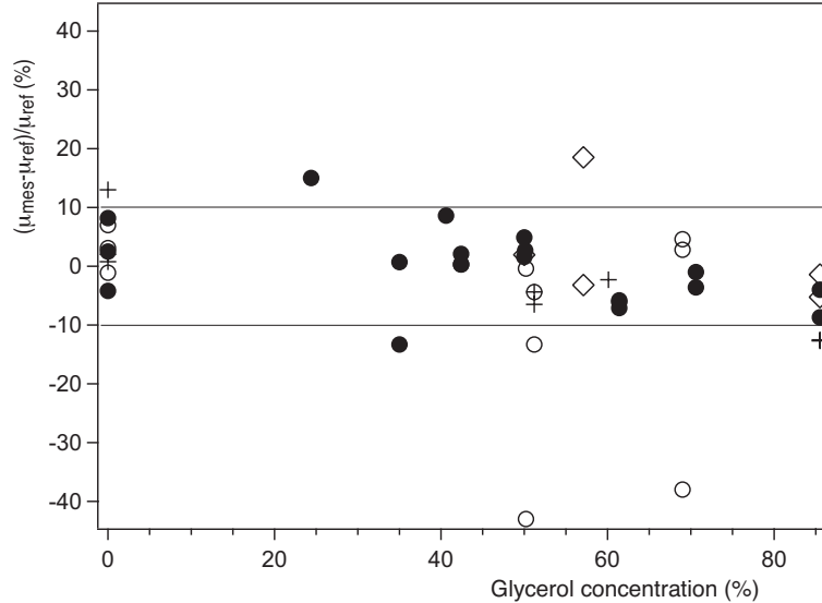
FIG. 8. Variations of the relative difference (\mu_{mes} - \mu_{ref})/\mu_{ref} between the measured viscosity \mu_{mes} and the values from ref. [17] at the same temperature as a function of the mass concentration of glycerol. (●): device A; (○): device B; (+) Contraves™ Low-shear 30 rotating viscometer; (◇): MCR501 AntonPaar™ rheometer with a double gap Couette assembly (only for \mu \gtrsim 10\text{mPa}\cdot\text{s} ).
