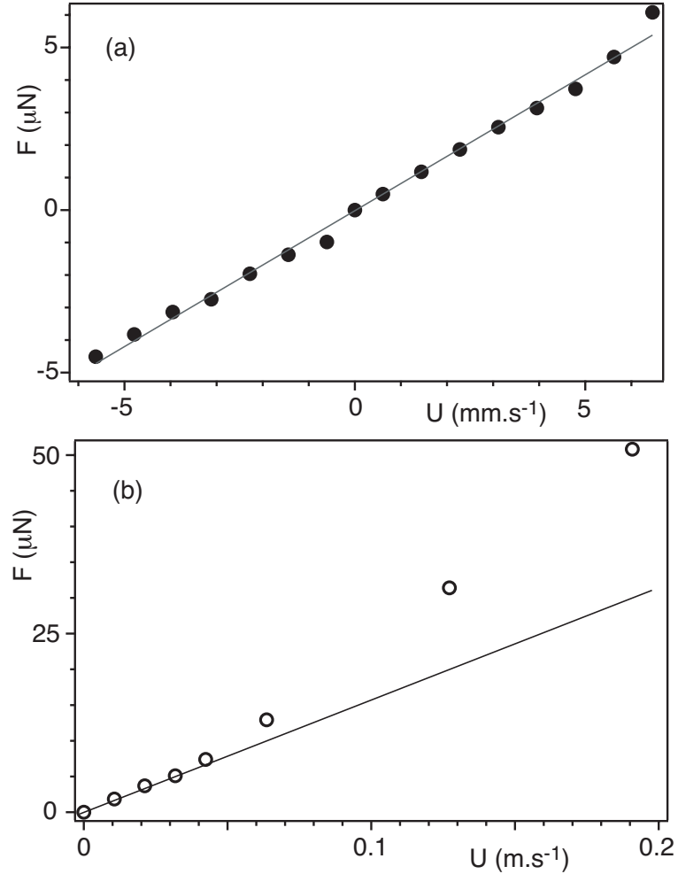
FIG. 4. Variation of the force on the cylindrical probe as a function of the mean velocity U of a water flow. (a) ( \bullet ): device A ( 0 \leq Re \leq 60 ); solid line: linear regression on all data of slope 0.715 \text{ g.s}^{-1} . (b) ( \circ ): device B ( 0 \leq Re \leq 200 ); solid line: linear regression on the first five points of slope 0.80 \text{ g.s}^{-1} .
