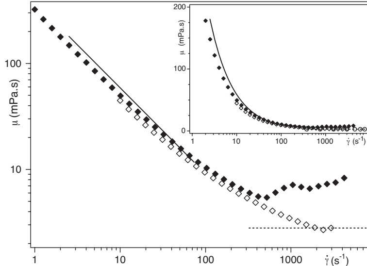
FIG. 10. Log-log plot of the dynamic viscosity \mu of a 1000 ppm scleroglucan solution at 23.6^\circ\text{C} as a function of \dot{\gamma} . The solid and dotted lines have the same meaning as in Fig. 9. ( \blacklozenge ) (resp. ( \diamond )) : Anton Paar MCR501 rheometer respectively in the cone plate and double gap configuration. Inset: lin-log plot of the same data.
