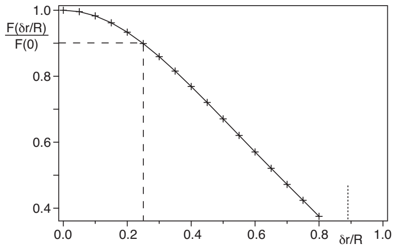
FIG. 3. Variation of the normalized force F(\delta r/R)/F(0) on the probe as a function of the normal transverse offset \delta r/R .
