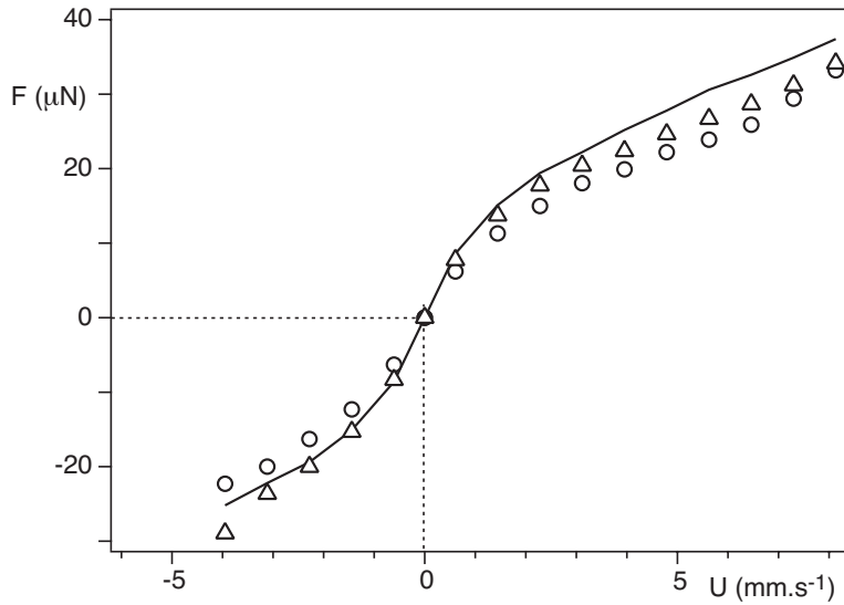
FIG. 5. Variation of the force F as a function of the mean flow velocity U for a 250 ppm polymer solution flowing in device A . ( \Delta ) and ( \circ ): measurements obtained for two consecutive tests. Solid line best theoretical fit of the experimental data in the case of a power law rheological characteristic: \mu = k\dot{\gamma}^\alpha .
