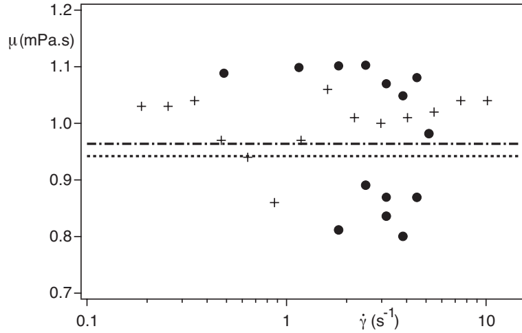
FIG. 6. Viscosity of pure water ( T = 22.6^\circ\text{C} ) measured using different devices. ( \bullet ): device A ; ( + ): Contraves Low-shear 30 rotating viscometer. Dotted line: value from Ref. [15]; Dashed dotted line, value obtained from a linear regression on the data of device A at different flow rates.
