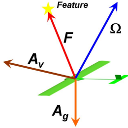
Fig. 2. The feature position ( \mathbf{F} ), the vehicle acceleration ( \mathbf{A}_v ) the vehicle angular speed ( \Omega ) and the gravity acceleration ( \mathbf{A}_g ).
