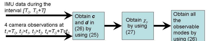
Fig. 3. The steps performed to estimate the observable modes when n_{obs} = 4 and in the case of one single feature.
