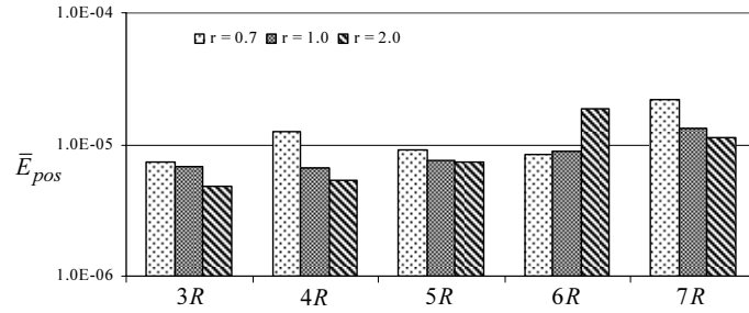
Fig. 3. \bar{P}_{error} of the nR -robot during n_C = 50 cycles for n = \{3, 4, 5, 6, 7\} and r = \{0.7, 1.0, 2.0\} .
