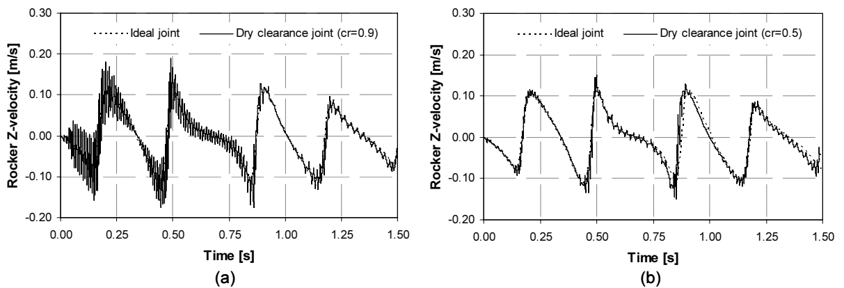
Figure 10. Influence of the restitution coefficient on the Z-rocker velocity of the four bar mechanism: (a) c_r=0.9 ; (b) c_r=0.5 .
