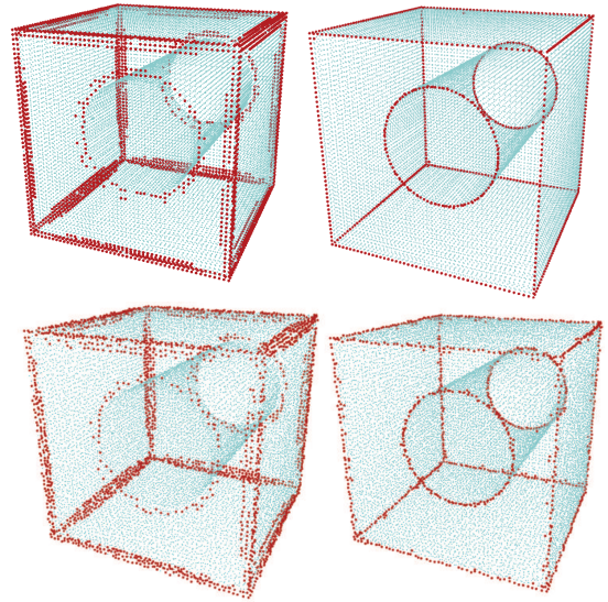
Fig. 18. Comparison of PCA-based feature detection (left) with our local-adaptive Gauss map clustering method (right). Both methods are applied to the original uniformly sampled point cloud of the cube-with-hole example (upper row) and to the perturbed data set with 1.2% of noise (lower row).
