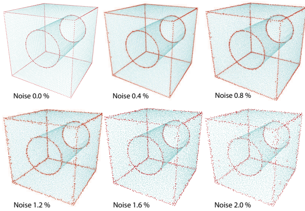
Fig. 12. Estimated feature points on noisy point clouds. The original cube-with-hole model is perturbed with random noise.
