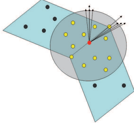
Fig. 1. Computation of the normal vectors used for feature identification in a local neighborhood.
