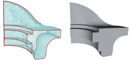
Fig. 14. Sharp feature detection on the fandisk model.
