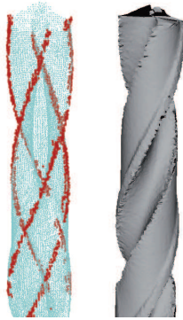
Fig. 17. Sharp feature detection on a drill scan by a Cyberware TM scanner. The data set is very rough and has missing data near the sharp feature.
