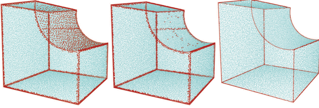
Fig. 8. The two pictures on the left show a non-uniformly sampled point cloud with an overrated set of feature points obtained with two different parameter settings \sigma = 0.1, k = 20 (left), \sigma = 0.5, k = 16 (middle). The right figure is the result obtained with the iterative method applied to the overrated examples. \sigma and k are automatically adapted for each of the feature candidates.
