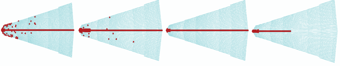
Fig. 6. Feature detection with a global sensitivity value \sigma . The points are sampled on a piecewise bilinear surface with a sharp feature line, similar to the example in Fig.7-left. The angle between the surfaces varies along the feature line from acute ( 45^\circ ) to obtuse ( 140^\circ ). The detected feature points are highlighted by fat red points. \sigma = 0.05, 0.1, 0.6, 1.0 left to right.
