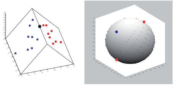
Fig. 3. Computation of the Gauss map G_p for feature identification in a local neighborhood.
