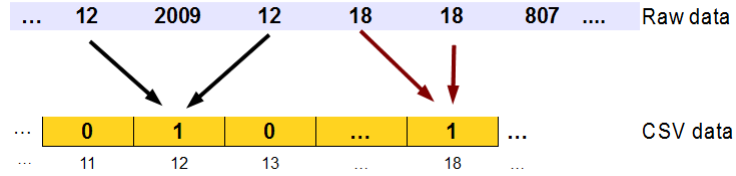
Figure 1: Example of formatting raw alert sequences into presence/absence data
