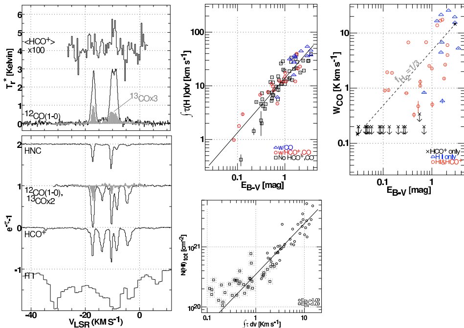
Fig. 1. Left: Example of the measurements available in emission (top) and in absorption (bottom) for one of the Galactic line of sight used in this study (for details see Pety et al., 2008). Middle, top: Integrated VLA HI optical depth from Garwood & Dickey (1989) and this work versus the total line of sight reddening from Schlegel et al. (1998). Middle, bottom: Total hydrogen column density versus integrated HI optical depth for the sources studied by Heiles & Troland (2003). Right: CO luminosity versus the total line of sight reddening from Schlegel et al. (1998).
