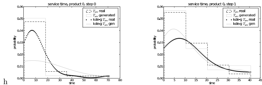
Figure 8: Service time. T_{srv} , distribution for two steps of a product for the experimental conditions presented in Table 3. The histogram of the original data ( T_{srv} real) is represented by the dashed line. The histogram regenerated by the application, for the same product and process step, is represented by the dotted line ( T_{srv} generated). Continuous estimation of the probability density function for the real (kde-g T_{srv} real, dots) and the generated case (kde-g T_{srv} gen, solid line) are made by the non-parametric method of kernel density estimation. Note that the estimation with kde is less accurate for service time than for the inter-arrival time, but the histogram estimation is robust.
