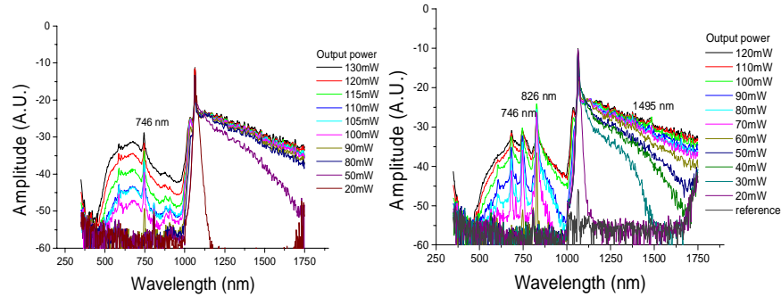
Fig. 3. Spectra generated in the MOF of 1.4 m versus coupled average power for polarization along the y axis (left) and the x axis (right).
