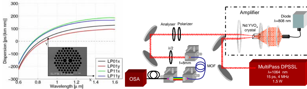
Fig. 1 (left). Numerically calculated dispersion of LP_{01x} , LP_{01y} , LP_{11x} , LP_{11y} modes of the birefringent fiber and its profile (inset). (Right). Experimental setup. DPSSL means Diode-Pumped Solid State Laser.
