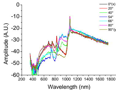
Fig. 2. Spectra generated in the MOF of 1.4 m versus polarization and for an output power of 120 mW.
