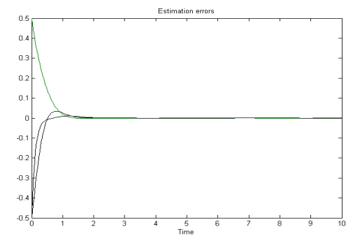
Fig.5. Estimation errors
