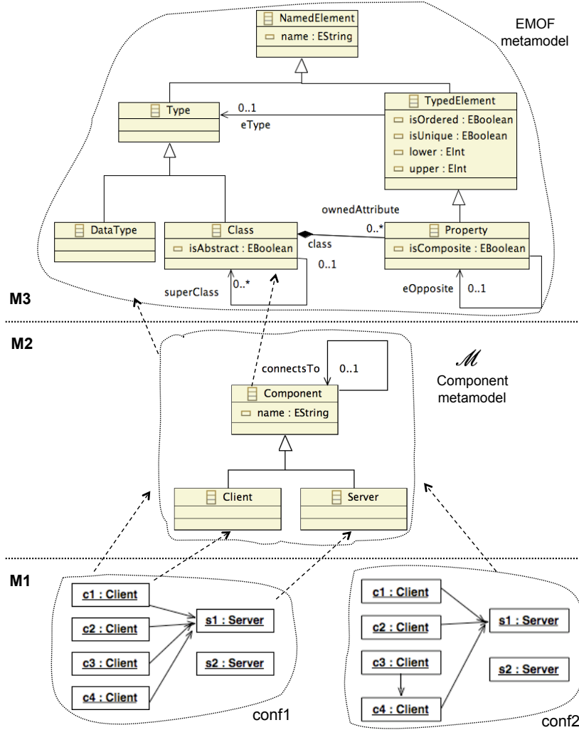
Fig. 1. The MOF framework.
