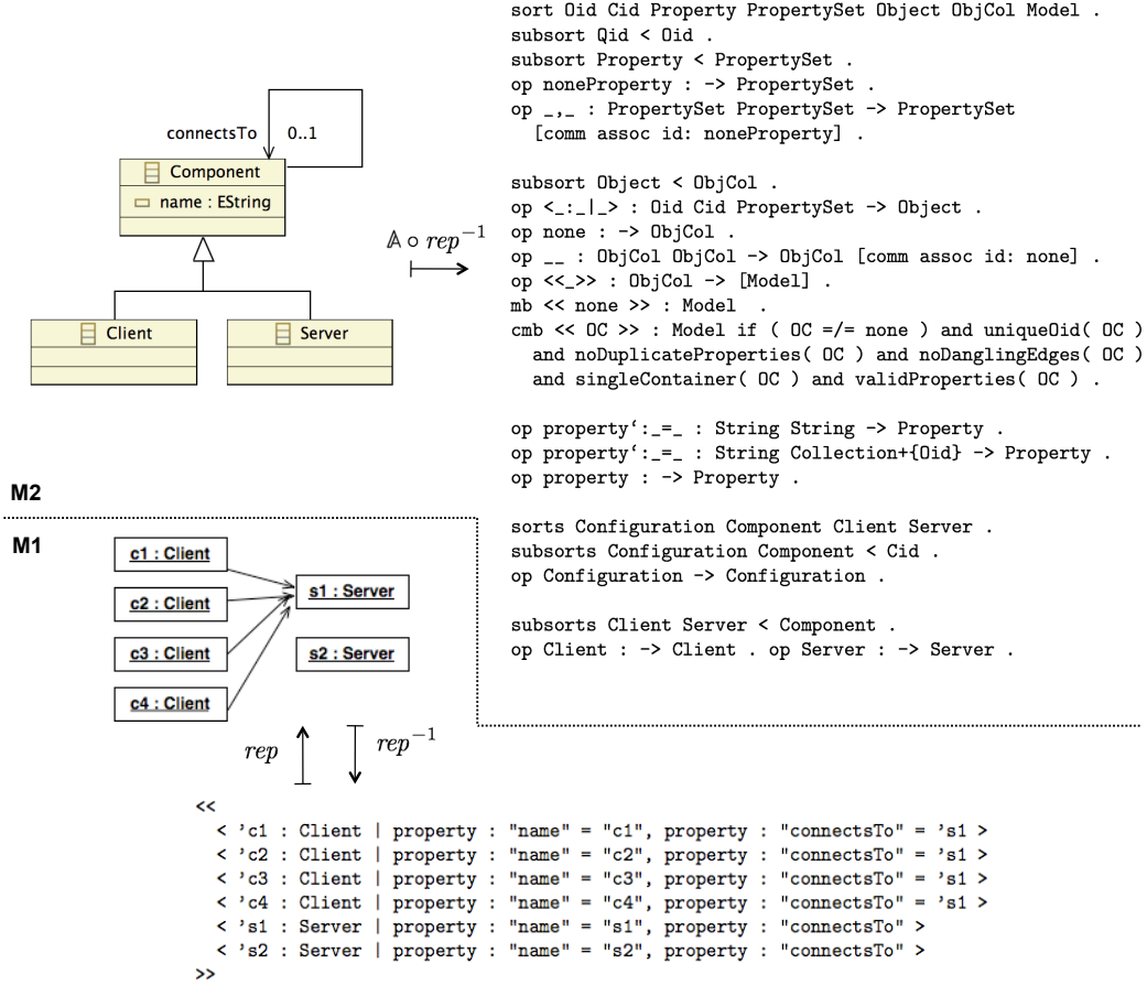
Fig. 3. EMF-Maude mappings in MOMENT2.
