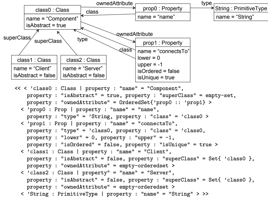
Fig. 2. Metamodel \mathcal{M} viewed as a graph and as a term.
