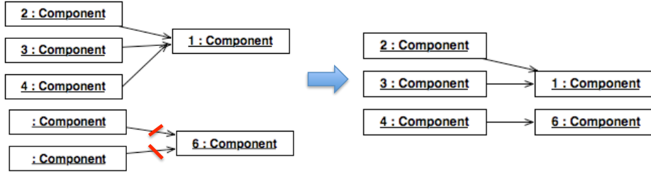
Fig. 5. Reconfiguration rule.
