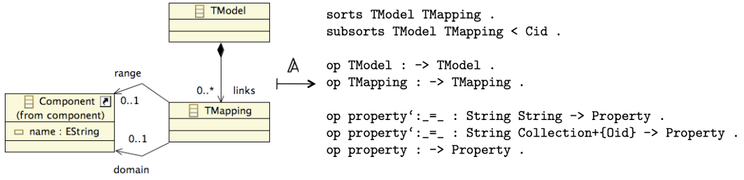
Fig. 6. Traceability metamodel \mathcal{T} and its algebraic realization \mathbb{A}(\mathcal{T}) .
