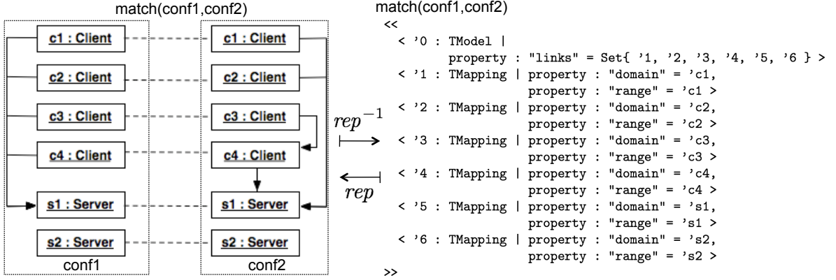
Fig. 7. Trace model and its term representation.
