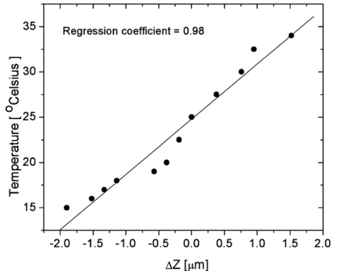
FIG. 3. Experimental beam position as a function of substrate temperature (circles) and the linear fit (solid line).
