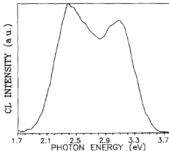
Fig. 8. CL spectrum of a small area of the \text{BaCuO}_2 ceramic.
