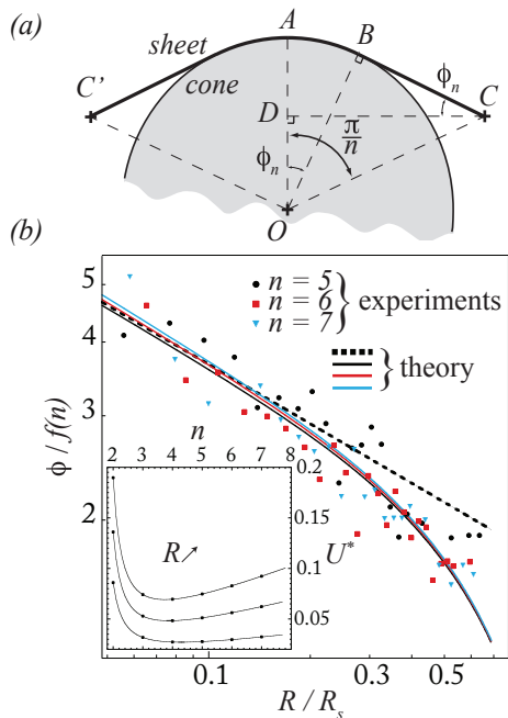
FIG. 3. (a) Schematic of the deformation of the inner boundary of the sheet in contact with the cone between crack tips located in C and C' . The folded petal is not shown. (b) Evolution of the angle \phi_n/f(n) with the perforation radius R/R_s . The solid line stands for the full theoretical prediction and the dotted line represents the approximation of Eq. (7). The dots stand for the measurements. Each experimental point represents the mean value of the 2n angles measured in a n cracks pattern. The inserted figure shows the evolution of the global energy U^* with cracks number n , computed for penetration radii 2 mm, 4 mm and 6 mm.
