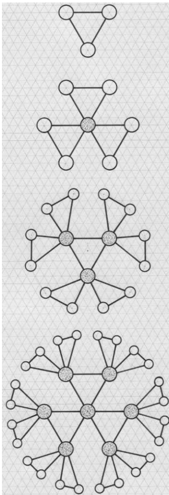
Figure 4: A compact illustration of the properties of the above-described finite geometries for (top to bottom) k = 2, 3, 4 and 5 . Each circle represents a doily and each triangle stands for a pencil of doilies; the filled circle means that the corresponding doily contains solely exceptional points.
