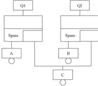
Figure 3 – Two Spare gates sharing a spare event
