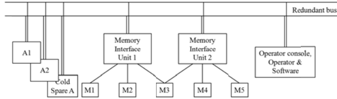
Figure 4 – The Computer System Example
