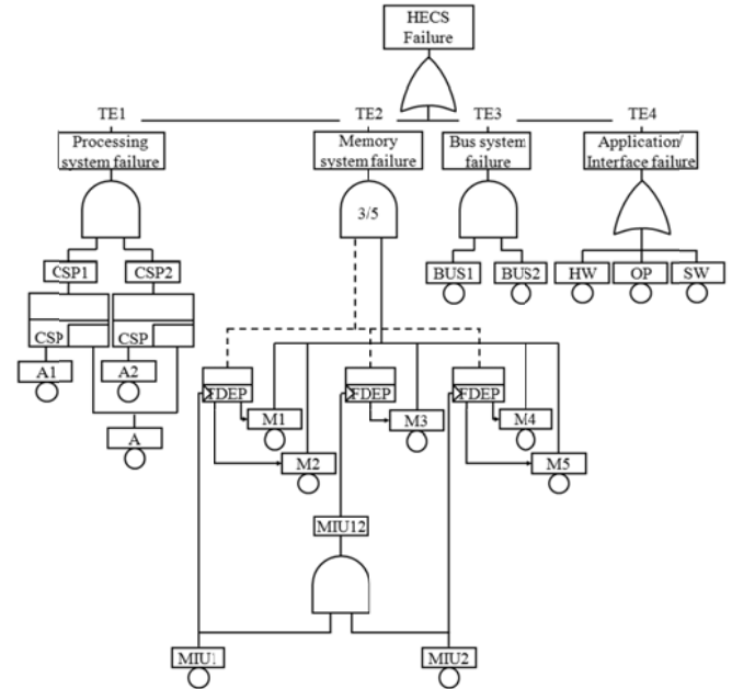
Figure 5 – The DFT of the HECS
