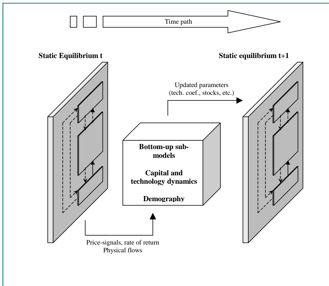
Figure 2 : The recursive dynamic framework of IMACLIM-R
