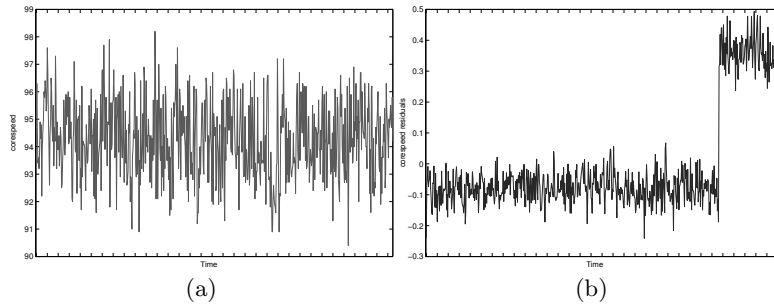
Fig. 1. (a) Rough measurements of the corespeed variable as a function of time for engine 6, (b) residuals of the same variable and for the same engine using a simple linear model with the environmental variables and the engine indicator as predictors (see Table 1).
