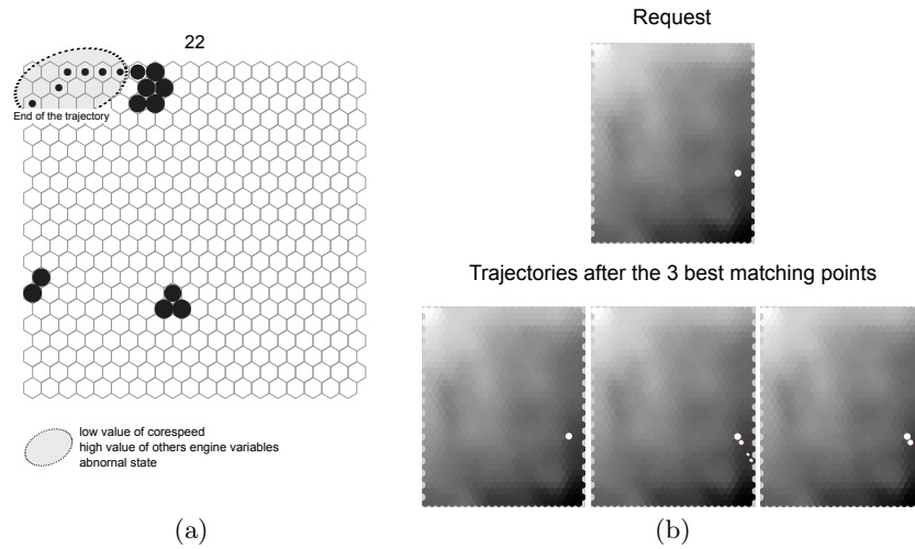
Fig. 5. Trajectories of engine 22 on the map. The sizes of the dots are proportional to the measurement date: smallest dots correspond to recent measurements, larger dots to older measurements.
