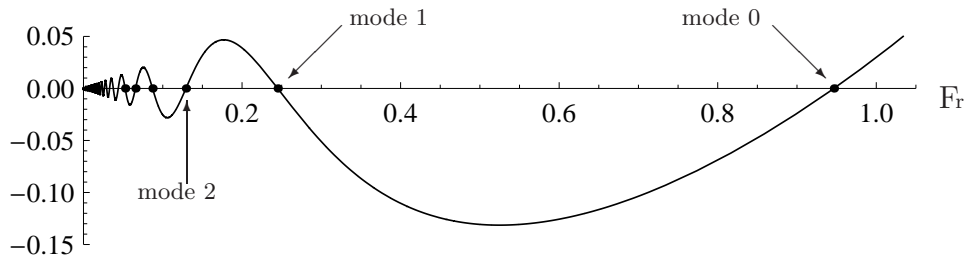
Figure 2: Graphical solution of the dispersion relation (37) with \varrho = 1 for long waves of infinitesimal amplitude in shallow water. Solid line represents the right-hand side function in Eq. (37); dots are the roots of that equation.
