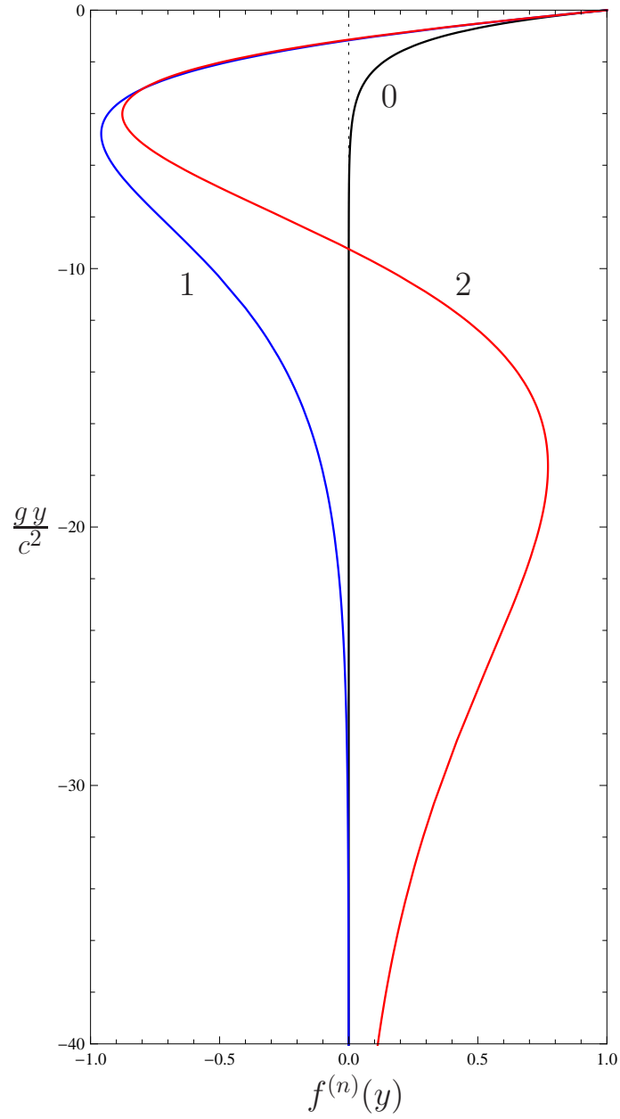
Figure 6: (color online) The first three eigenfunctions f^{(n)}(y) in the case of deep water for \text{Fd} = 1 . a): n = 0 ( K^{(0)} = 1 ); b): n = 1 ( K^{(1)} \approx 0.303 ); c): n = 2 ( K^{(2)} \approx 0.188 ). All eigenfunctions are normalized such that f^{(n)}(0) = 1 [see Eq. (22)].
