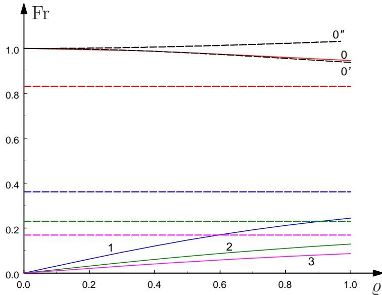
Figure 3: (color online) Froude number against the stratification parameter \varrho for the first four modes of infinitely long waves. The surface mode is labeled by 0, and first three internal modes are labeled by numbers 1, 2, 3. Line 0' shows the asymptotic dependence for the surface mode when \varrho \rightarrow 0 , and line 0'' shows the asymptotic dependence for the surface mode when Fr \rightarrow 0 . The color dashed horizontal lines show the asymptotic values of corresponding dispersion lines when \varrho \rightarrow \infty .
