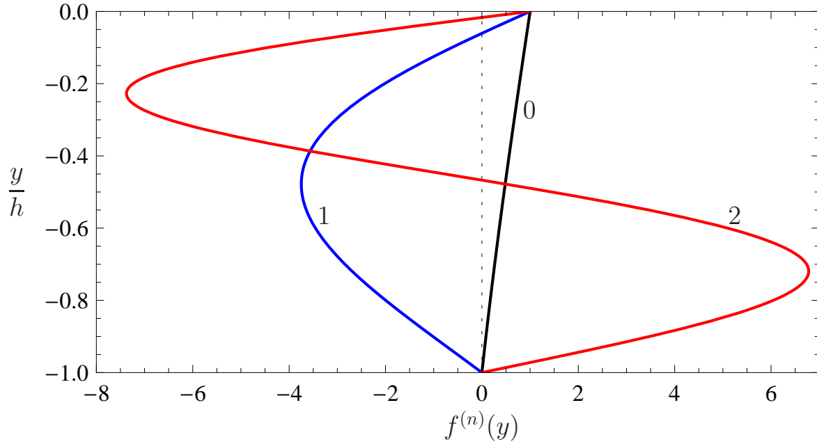
Figure 4: (color online) The structure of the first three modes of infinitely long waves in linear stratification (15) for \varrho = 1 . The numbers in the plots indicate the mode numbers.
