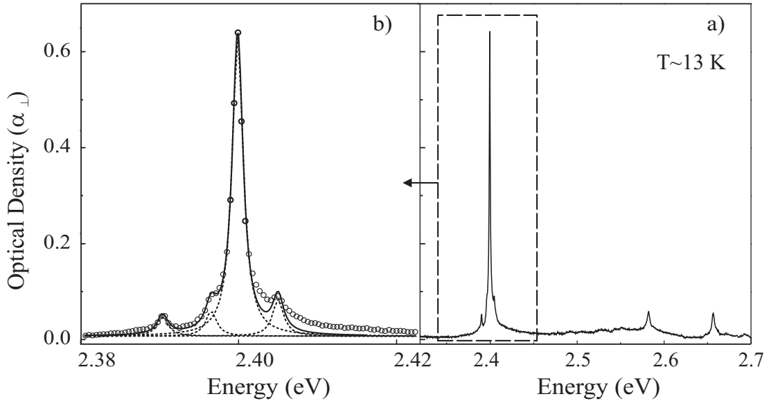
FIG. 4: a) Absorption spectrum, \alpha_{\perp} , at 13 K of a crystal with x_p \sim 8 \times 10^{-4} for an incident field polarized perpendicular to the chain direction. b) Detail of the exciton line: experimental data (open circles), fit (solid line) and lorentzian contributions to the fit (dashes).
