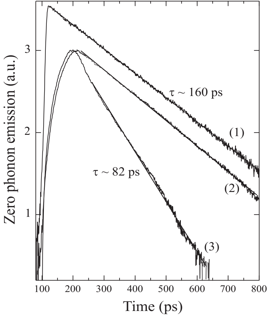
FIG. 8: Temporal decay at 6.5 K of the poly-3NPh2 zero phonon emission. (1) and (2): Zero phonon “broad” emission (II); (3) dynamics of the “narrow” emission (I). Curve (1) is obtained using a twelve times less dispersive grating (100 lines/mm). The pump power is always less than 50 nW.
