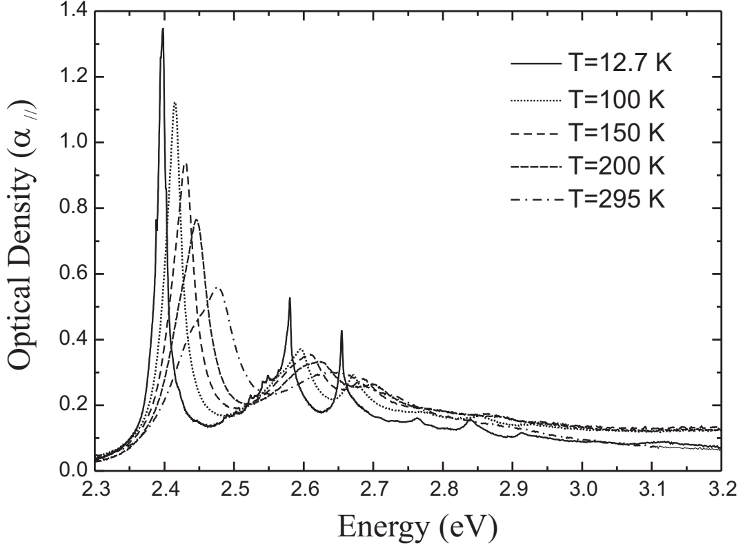
FIG. 3: Temperature dependence of the optical absorption, \alpha_{//} (incident electric field parallel to the \mathbf{a} -axis), of isolated poly-3NPh2 chains in their host crystal ( x_p \sim 4 \times 10^{-5} ). The sample thickness e \sim 440 \mu\text{m} leads to an absorption constant at the signal maximum, \alpha_{max} \sim 72 \text{ cm}^{-1} at 12.7 K.
