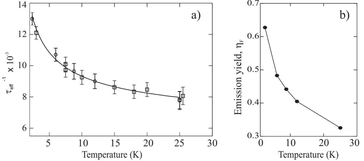
FIG. 9: Plot of \tau_{eff}^{-1} versus temperature for the narrow emission (I) at 2.401 eV. Two series of data are plotted (opened circles and squares). The solid line is the result of a fit \tau_{eff}^{-1} = \tau_{nr}^{-1} + 1/b\sqrt{T} . b) Calculated quantum yield of emission deduced from the adjustment of \tau_{rad} .
