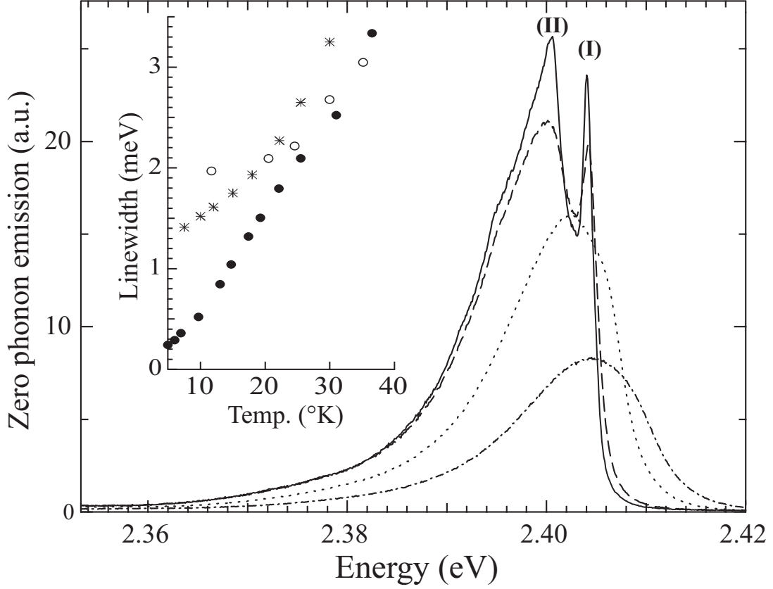
FIG. 7: Zero phonon emission of poly-3NPh2 chains at 8 K (solid line), 18 K (dashed line), 30 K (dotted line) and 60 K (dash-dotted line). Inset: Temperature dependence of the linewidth of different polydiacetylene chains: isolated poly-3NPh2 in crystals with x_p \sim 3 \times 10^{-5} in weight (stars), ensemble of isolated poly-3BCMU chains x_p \sim 3 \times 10^{-5} (open circles) and single poly-3BCMU chains at x_p \sim 3 \times 10^{-7} (filled circles).
