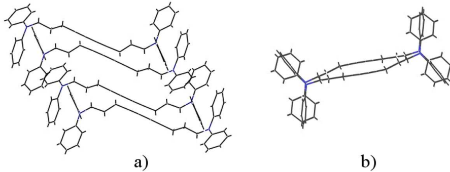
FIG. 1: Crystal structure of the 3NPh2 diacetylene: a) Two pairs of non equivalent monomers; b) The same pairs as in a) but viewed along the polymerization direction ( a axis), perpendicular to the plane of the figure.
