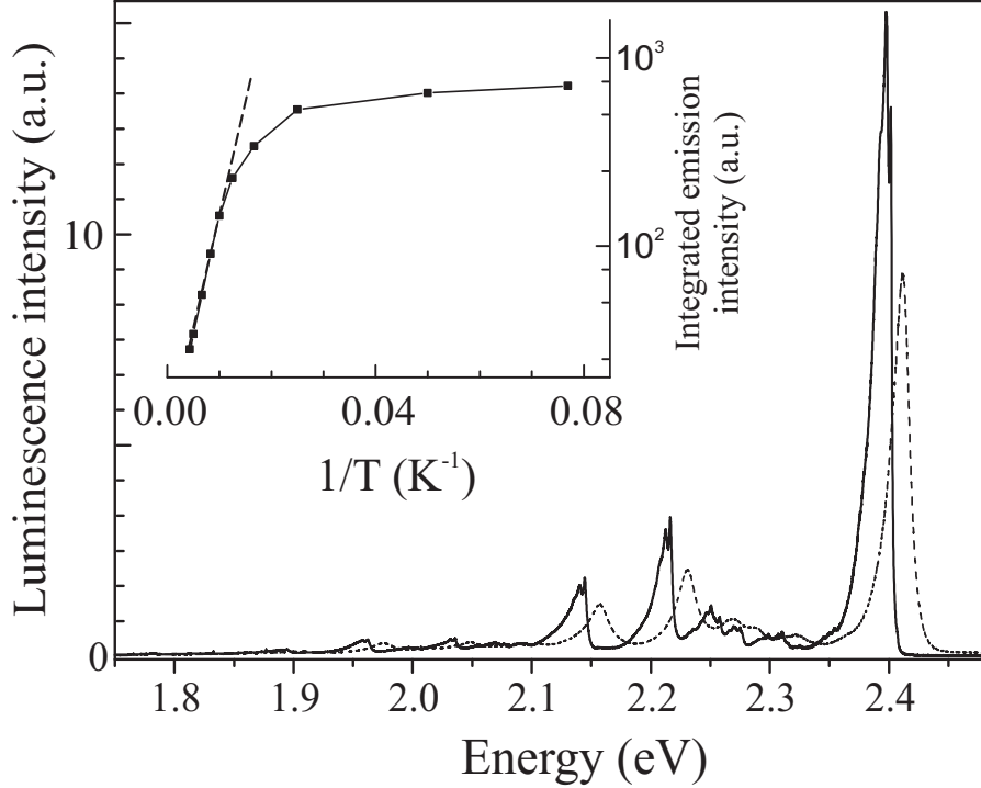
FIG. 6: : Emission of isolated chains of poly-3NPh2 at 8 K (solid line) and 55 K (dashed line). Inset: Arrhenius-like plot of the integrated emission intensity (solid line) and associated fit for T > 60K (dashes) giving an activation energy E_{act} \sim 22 meV.
