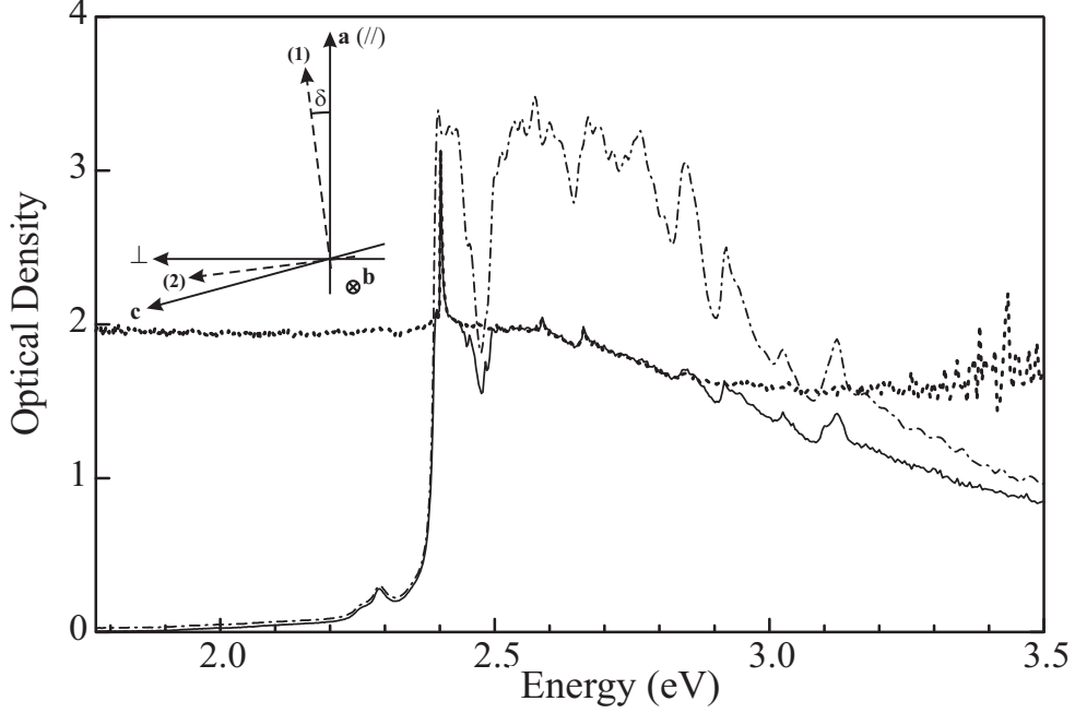
FIG. 5: Absorption spectra, at 13 K, of a crystal with x_p \sim 1.4 \times 10^{-3} for different configurations of the polarizer and analyzer. Dash-dotted line: //-/// configuration; solid line: //-(\text{no analyzer}) configuration; dots: //-\perp configuration. Inset: geometrical configuration for absorption spectroscopy of 3NPh2 crystals. a , b , c are the crystallographic axis. (1) and (2) are two of the principal axis of [\epsilon_1] ; b is the third principal direction in a monoclinic crystal. \delta is the angle between a and (1). In the experiments the incident light is perpendicular to the (a,c) plane and polarized either parallel ( // ) or perpendicular ( \perp ) to a .
