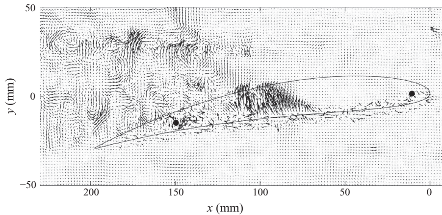
FIGURE 22. Averaged tip-flow field statistically related to the largest high-frequency pressure fluctuations in the far field.
