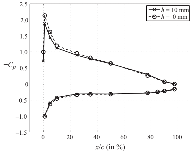
FIGURE 4. Example of pressure coefficient distribution along the pressure and suction sides of the aerofoil for the self-noise and the maximum gap configuration.
