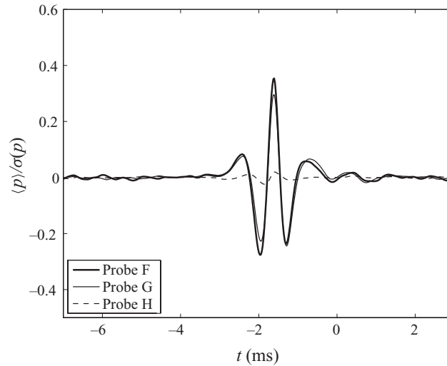
FIGURE 9. Averaged pressure time signatures obtained in the trailing-edge region ( x/c = 0.975 ) for the reference gap configuration: effect of the distance from the gap ( z ): probe F ( z/c = 0.005 ), probe G ( z/c = 0.015 ) and probe H ( z/c = 0.03 ). The amplitudes are normalized with respect to the standard deviation of the original signals ( \sigma_p ).
