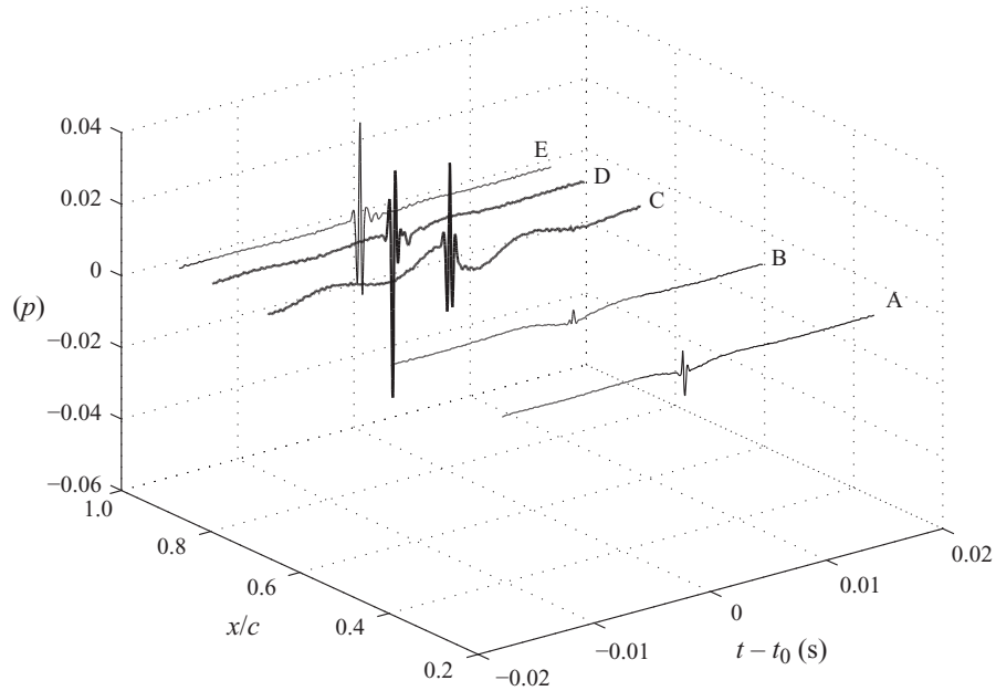
FIGURE 8. Averaged pressure time signatures obtained for several chordwise positions in the tip region ( z/c = 0.005 ) for the reference gap configuration. From right to left: probe A ( x/c = 0.25 ), probe B ( x/c = 0.50 ), probe C ( x/c = 0.775 ), probe D ( x/c = 0.90 ) and probe E ( x/c = 0.955 ).
