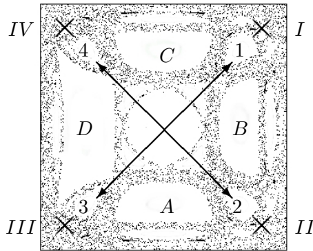
Figure 12: Sketch of the velocity field for the Poincaré section corresponding to protocol A, \alpha = 1.8 in the square: during stage 1 (respectively 2, 3 or 4), the sink is the hole located at cross I (respectively II , III or IV ), the source is the hole located at the cross at the opposite corner.
