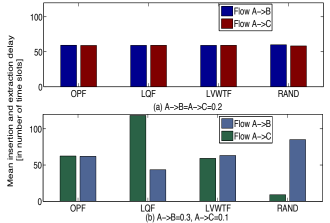
Fig. 2. Comparison of scheduling mechanisms in scenario from Fig. 1, for k = 1
