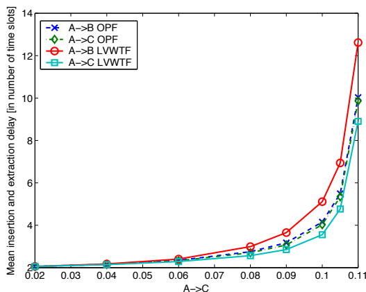
Fig. 3. LVWTF versus OPF in 2-wavelength receiver ring: A \rightarrow B = 2 \cdot (A \rightarrow C)
