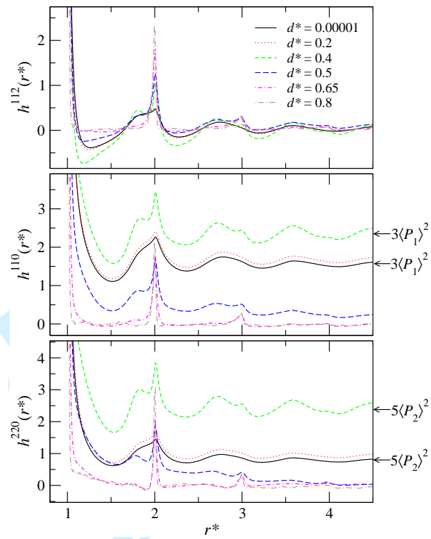
Figure 6. Projections h^{112}(r^*) , h^{110}(r^*) , and h^{220}(r^*) of the pair-correlation function for a high density ( \rho^* = 0.8 ) for various values of d^- .
