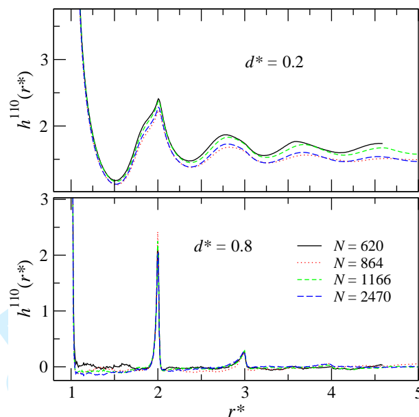
Figure 9. System size dependence of the projection h^{110}(r^*) for various values of d^* at high a density ( \rho^* = 0.8 ) using tin-foil boundary condition ( \epsilon_{RF} \rightarrow \infty ). Various lines represent various numbers of particles as indicated in the figure.
