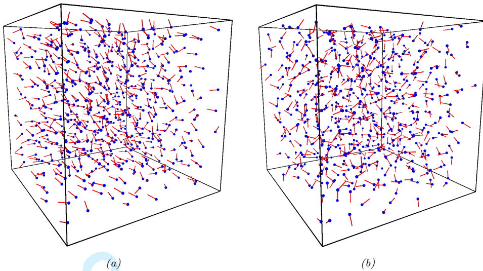
Figure 7. Snapshot of randomly chosen configurations for (a) d^* = 0.2 and (b) d^* = 0.8 at a high density ( \rho^* = 0.8 ). Blue dots represent the centers of the spheres, while the red rods show the orientations of the dipoles.
