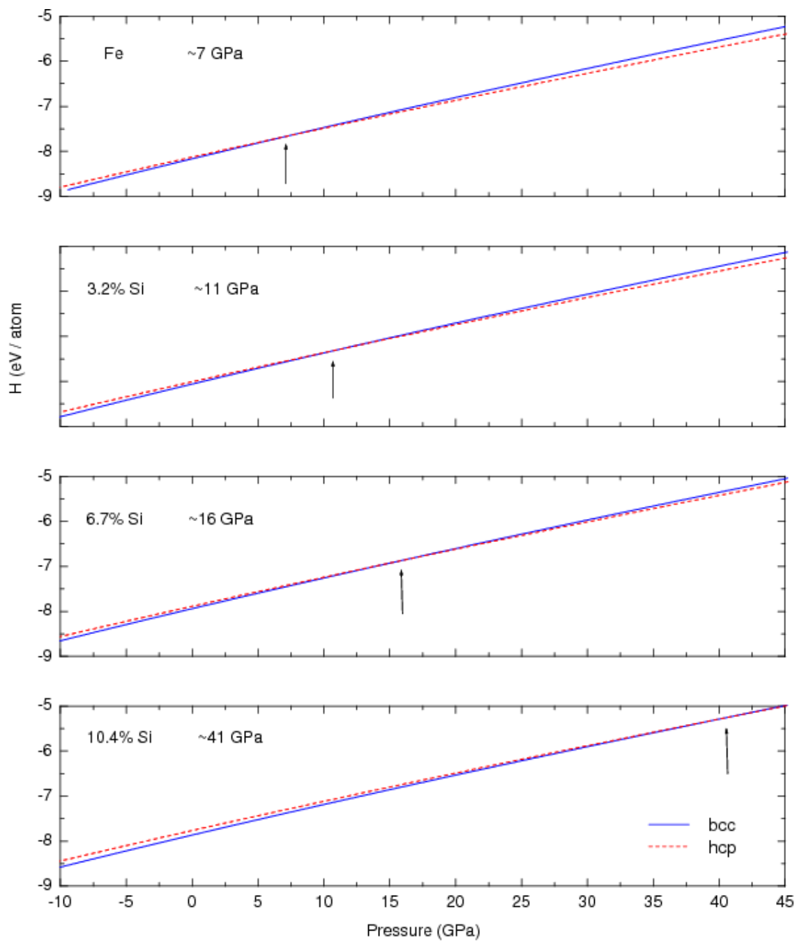
Figure 2: Calculated enthalpy curves for bcc and hcp structures at 3 different concentrations of silicon. The arrows indicate the transition pressures for the pseudo-univariant reactions.
