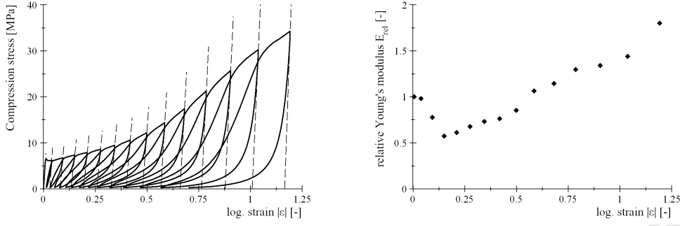
a) b) Fig. 15. Investigation of compression damage: a) Uniaxial cyclic loading and unloading; b) Relative Young's modulus
