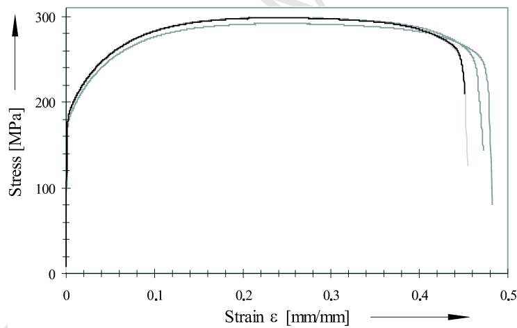
Fig. 18. Stress strain curve of the steel DC01
