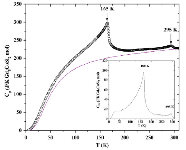
Fig. 6. Temperature dependence of the heat capacity C_p of \text{Gd}_5\text{CoSi}_2 (annealed sample) between 5 and 310 K. The line represents the sum of the electronic ( \gamma=100 \text{ mJ mol}^{-1} \text{ K}^{-2} ) and lattice ( \theta_D=210 \text{ K} ) contributions. Inset shows the temperature dependence of the magnetic contribution C_m .
