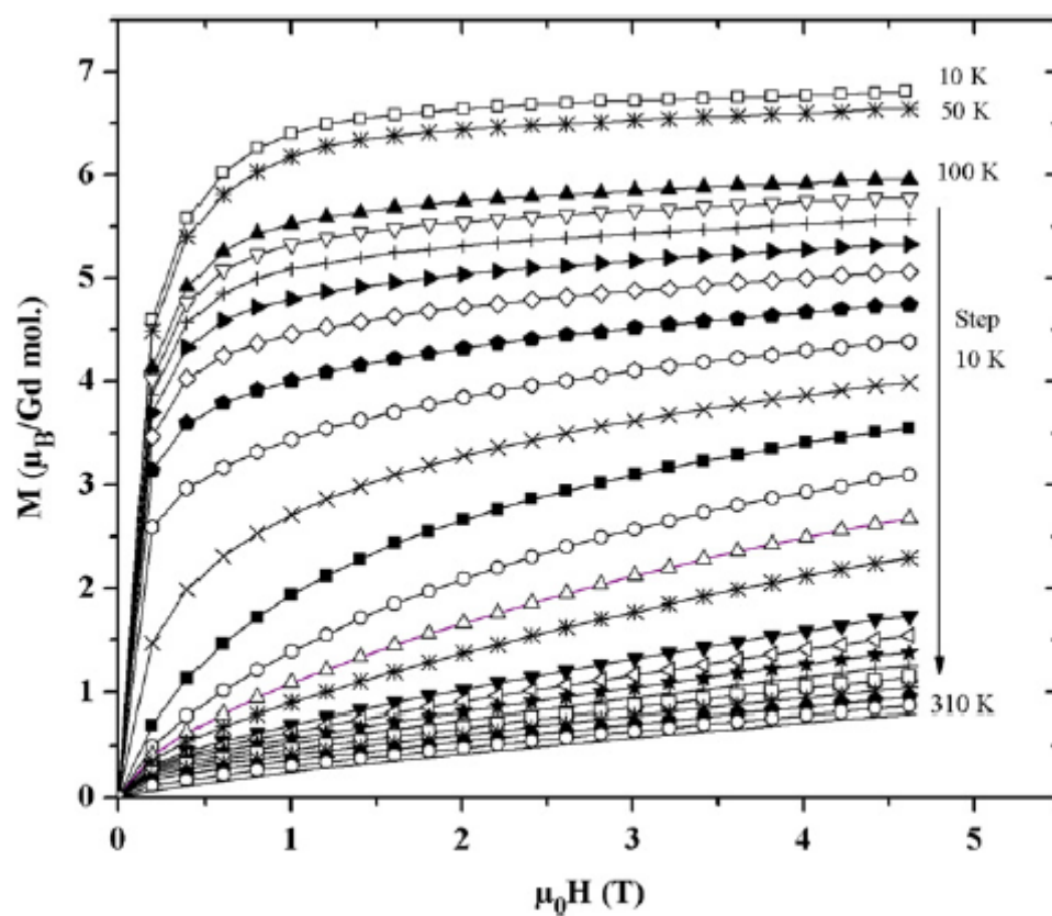
Fig. 8. Field dependence of the magnetization M of \text{Gd}_5\text{CoSi}_2 (annealed sample) measured at various temperatures.
