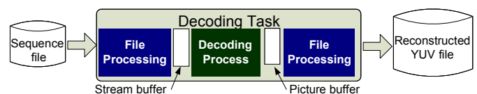
Fig. 9. DSP-based Open SVC decoder testbench.
