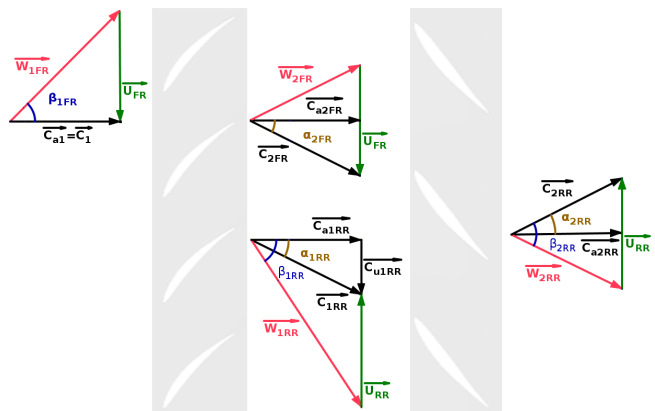
FIG. 2. Velocity Triangles for the CRS. The fluid is flowing from left to right. Please see the Nomenclature for the meaning of the capital letters and subscripts. Please also note that this is a general case where the exit-flow is not constrained to be solely axial
