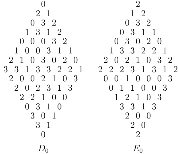
Figure 3: The building blocks of \nabla S_1[8k] (continued)
