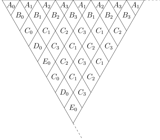
Figure 2: Structure of \nabla S_1[8k]
