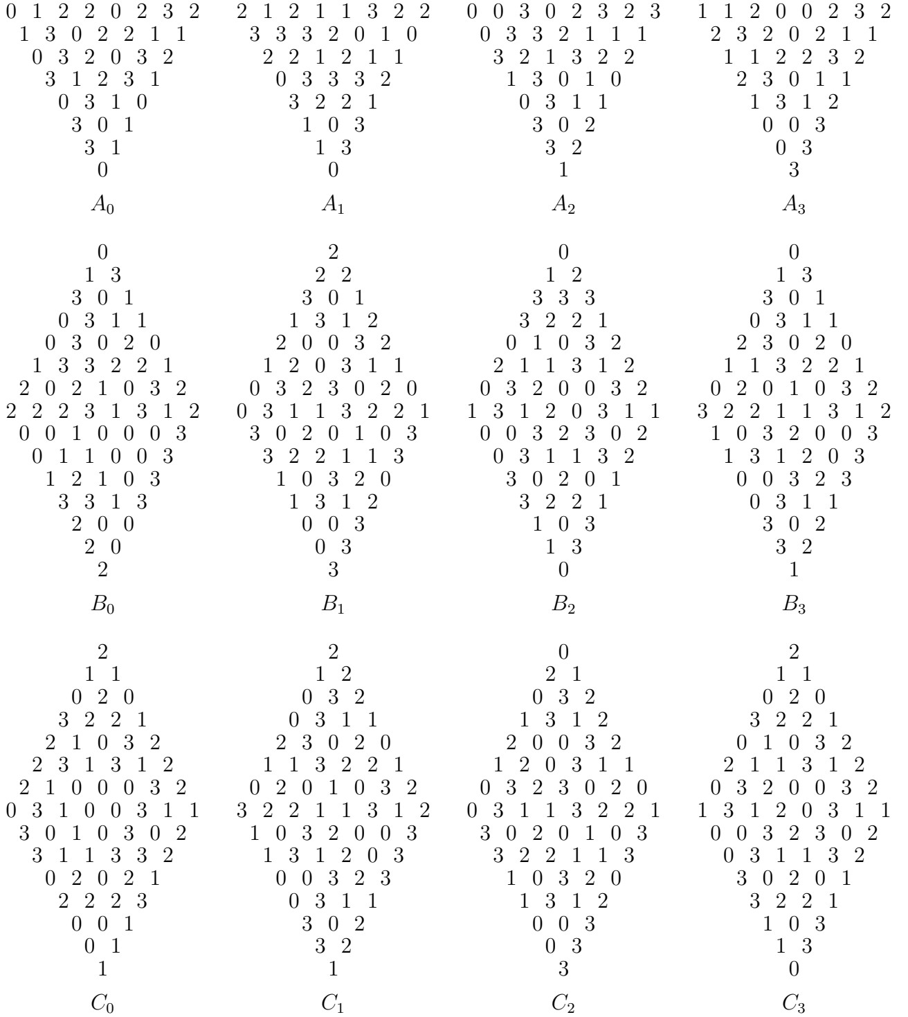
Figure 3: The building blocks of \nabla S_1[8k]
