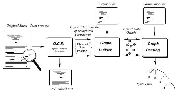
Figure 1: The Ofr architecture
