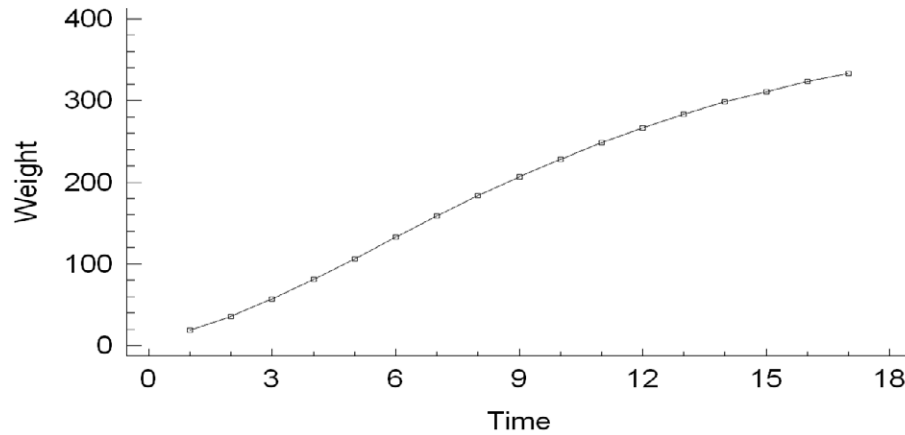
Figure 2. Mean weight to age for swordfish in both sexes.
