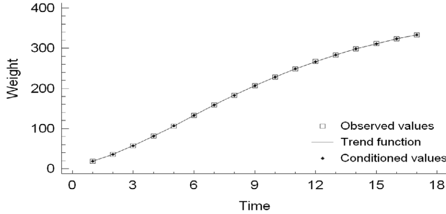
Figure 3. Observed values and estimations of the trend function and the E[X(t_i)|X(t_{i-1}) = x_{i-1}] values, i = 1, \dots, 17 .
