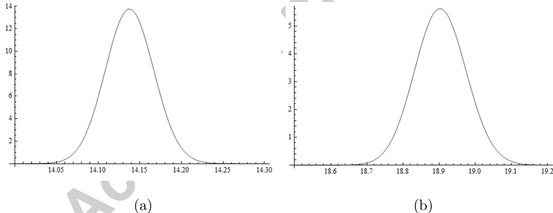
Figure 4. First-passage probability densities for the weight of the swordfish through a constant boundary: (a) S = 300 ; (b) S = 350 .
