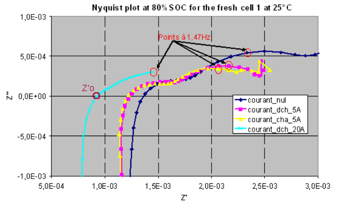
Figure 8-b: zoom on the Nyquist plot of Figure 6-a
