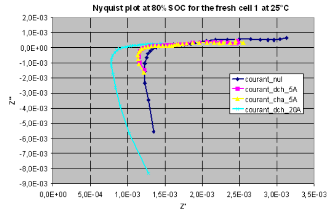
Figure 8-a: results of EIS measurement for VL6P Cell 1
