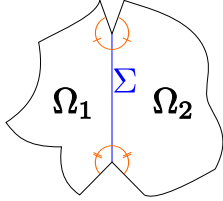
FIGURE 7. A is Fredholm of index 0 when \sigma_2/\sigma_1 \in \mathbb{R}_-^* \setminus \{-1\} .
