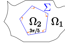
FIGURE 10. A is Fredholm of index 0 when \sigma_2/\sigma_1 \in \mathbb{R}_-^* \setminus [-7/3; -3/7] .
