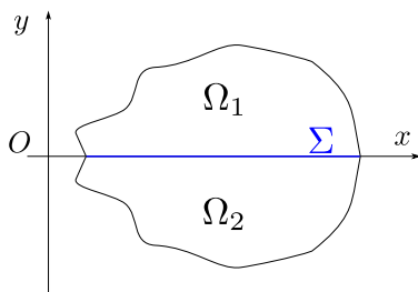
FIGURE 1. A symmetric geometry.
