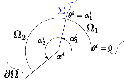
FIGURE 5. Notations for \mathbf{x}^i \in \mathcal{S}_{ext} - \alpha^i = \alpha_1^i .
