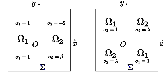
FIGURE 11. Two situations not covered by theorem 3.3: \beta > -1 on the left; \lambda \in \mathbb{R}_* on the right.
