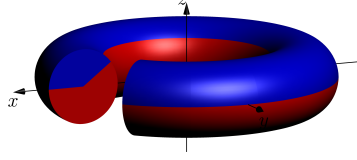
FIGURE 13. Geometry of an interior axisymmetric edge.
