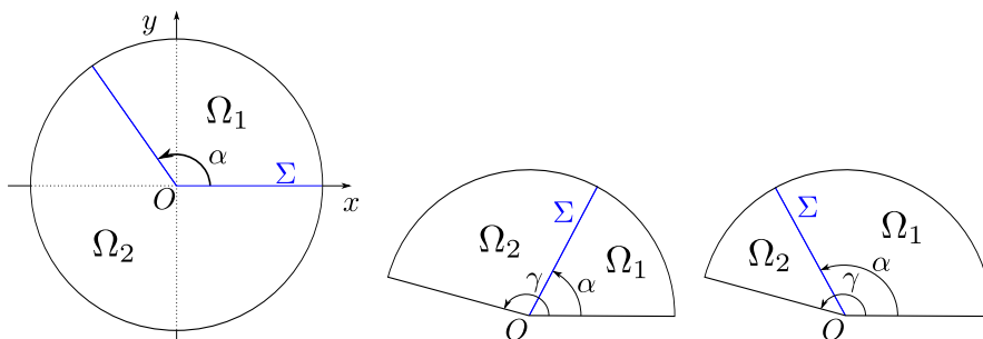
FIGURE 2. (Left) Geometry of an interior vertex. (Middle, right) Geometries of a boundary vertex.
