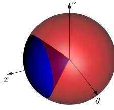
FIGURE 14. Geometry of an interior conical vertex.
