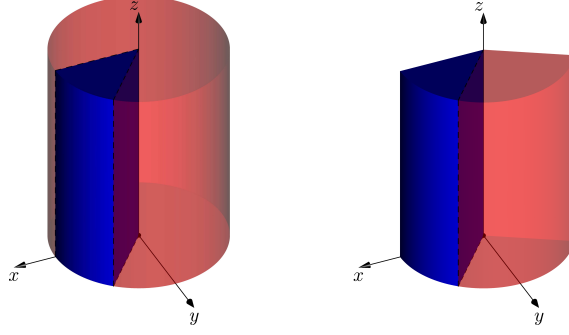
FIGURE 12. Geometry of prismatic edges: (left) interior edge. (Right) boundary edge.
