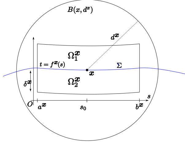
FIGURE 6. Situation in a neighborhood of \mathbf{x} .
