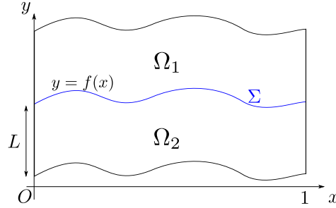
FIGURE 3. Geometry for an interface of \mathcal{C}^1 -class.
