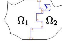
FIGURE 8. A is Fredholm of index 0 when \sigma_2/\sigma_1 \in \mathbb{R}_-^* \setminus [-3; -1/3] .
