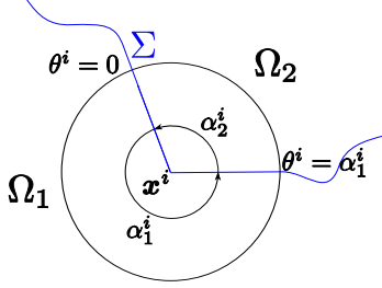
FIGURE 4. Notations for \mathbf{x}^i \in \mathcal{S}_{int} - \alpha^i = \alpha_2^i .
