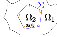
FIGURE 10. A is Fredholm of index 0 when \sigma_2/\sigma_1 \in \mathbb{R}_-^* \setminus [-7/3; -3/7] .
