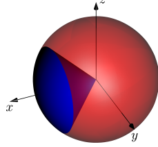
FIGURE 14. Geometry of an interior conical vertex.
