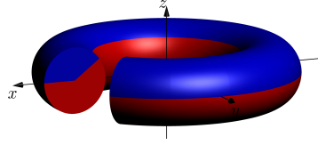
FIGURE 13. Geometry of an interior axisymmetric edge.
