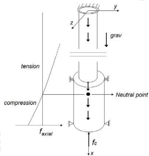
Figure 6: Initial prestressed configuration of the system.
