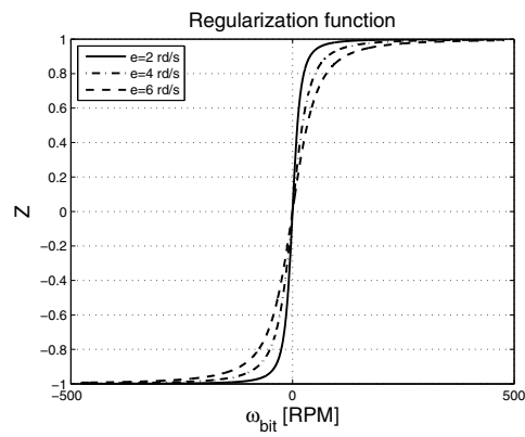
Figure 3: Regularization function.
