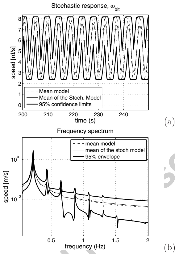
Figure 10: Stochastic response for \delta = 0.001 . Rotational speed of the bit (a) and its frequency spectrum (b).
