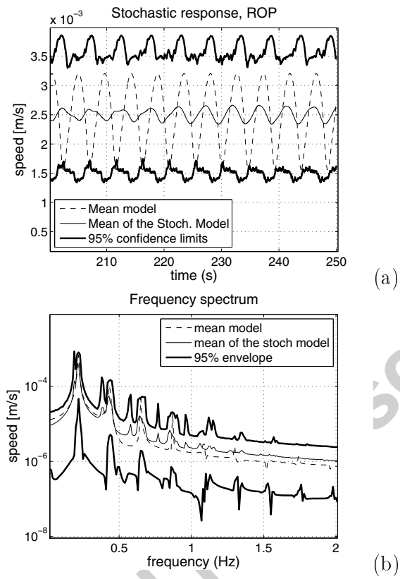
Figure 12: Stochastic response for \delta = 0.01 . ROP (a) and its frequency spectrum (b).
