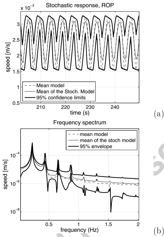
Figure 8: Stochastic response for \delta = 0.001 . ROP (a) and its frequency spectrum (b).
