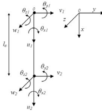
Figure 2: Degrees of freedom of an element.
