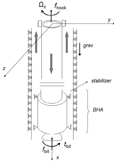
Figure 1: General scheme of the drill-string system.
