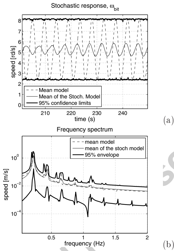
Figure 13: Stochastic response for \delta = 0.01 . Rotational speed of the bit \omega_{bit} (a) and its frequency spectrum (b).
