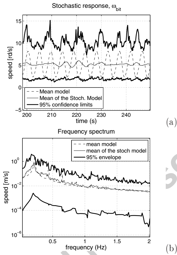
Figure 15: Stochastic response for \delta = 0.1 . Rotational speed of the bit \omega_{bit} (a) and its frequency spectrum (b).
