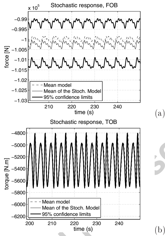
Figure 9: Stochastic response for \delta = 0.001 . (a) weight-on-bit, (b) torque-on-bit.
