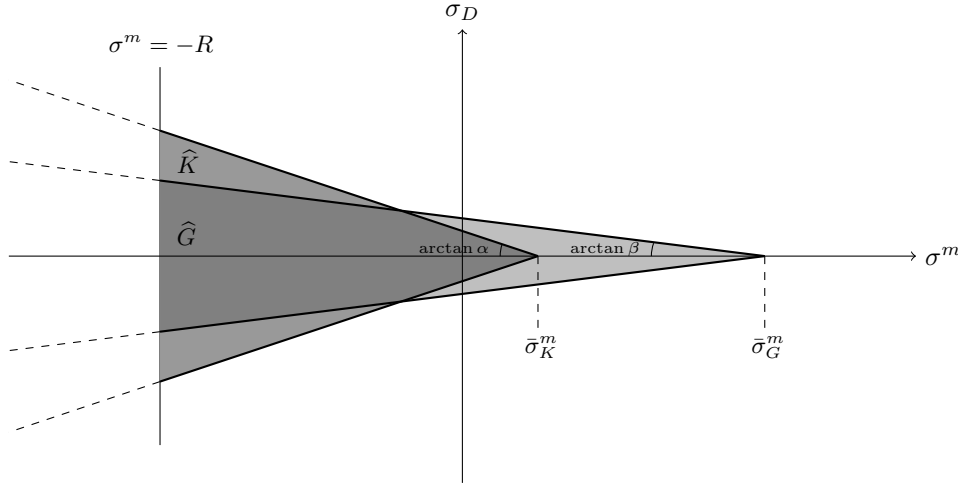
FIGURE 1. The sets \hat{K} and \hat{G} .
