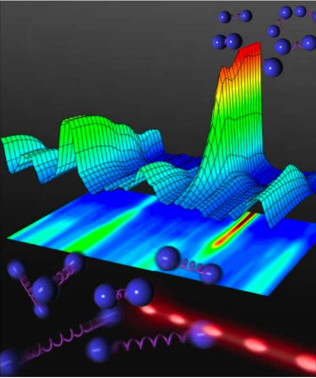
FIG. 2. Illustration of the optical pumping of molecules using train of shaped laser pulses. As times goes on (from bottom-left to up-right) the vibration of the molecules is modified by the laser pulses: all molecules end up in the same non vibrating state. The experimental signal, adapted from reference [264], shows the temporal evolution of the populations in the different vibrational levels of the ground state. The decreasing populations correspond to vibrational states v = 1 - 10 whereas the increasing signal corresponds to the population of v = 0 .
