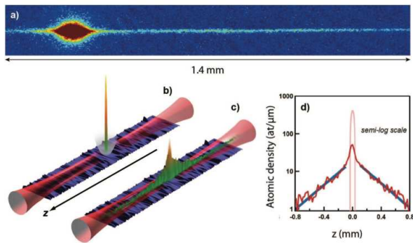
FIG. 1. Top (a): Image by absorption of an atom laser directly outcoupled in an horizontal optical waveguide (from ref. [127]). Bottom: Experimental scheme of [36] for the demonstration of Anderson Localisation with ultracold atoms. Following the proposal [148], a somewhat crude version of an atom laser (the whole initial BEC (b) being released) is allowed to expand along a guide and is stopped in presence of a laser speckle disorder (c). d) Density profile of the stationary state in semi-log scale. The exponential decay observed in the wing is the emblematic signature of Anderson Localisation [149].
