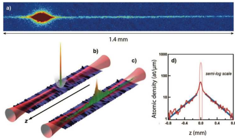
FIGURE 1: Top (a) : Image by absorption of an atom laser directly outcoupled in an horizontal optical waveguide (from ref. [86]). Bottom : Experimental scheme of [34] for the demonstration of Anderson Localization with ultracold atoms. Following the proposal [107], a somewhat crude version of an atom laser (the whole initial BEC (b) being released) is allowed to expand along a guide and is stopped in presence of a laser speckle disorder (c). d) Density profile of the stationary state in semi-log scale. The exponential decay observed in the wing is the emblematic signature of Anderson Localization [108].
