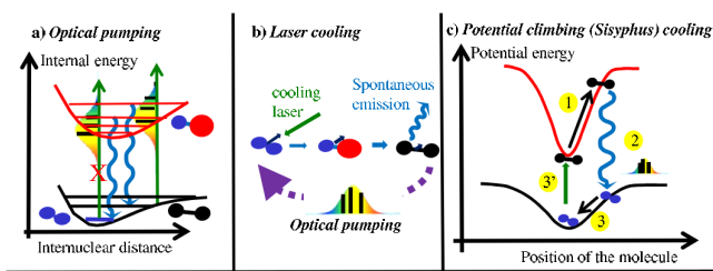
FIGURE 2: a) Principle of laser cooling of molecules through absorption-spontaneous emission cycles to transfert (photon) momentum; if needed (dashed line) an optical pumping step can be added. b) Principle of "one-way" or "Sisyphus cooling" of molecules : 1) remove kinetic energy through motion in an external potential, 2) dissipative process avoiding the reverse motion, 3) if needed the process can be repeated by bringing the molecule back, in position using the trapping potential, and in its original internal state using light absorption.
