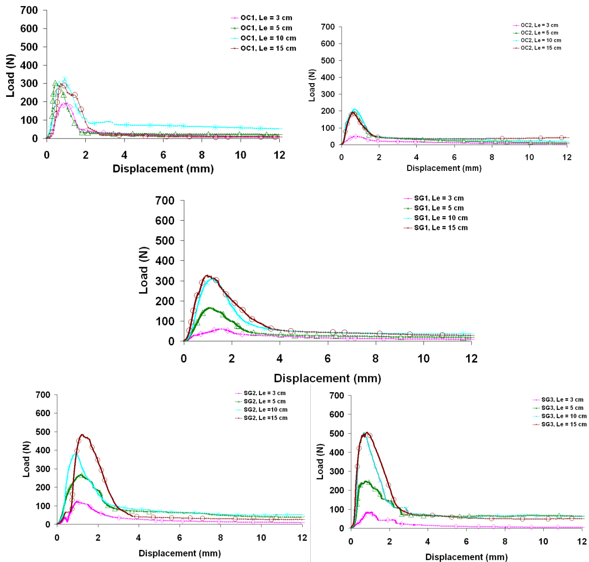
Figure 2. Load pull-out versus displacement of means curves.
