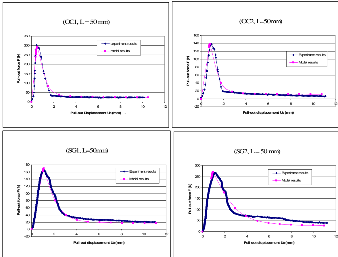
Figure 4. Pull-out curve for different types of fiber.
