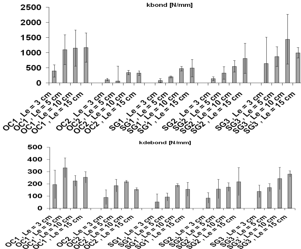
Figure 5. Bonding and debonding parameters between multi-filaments yarn / cementitious matrix.
