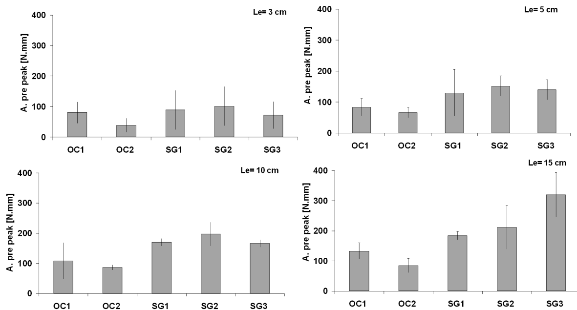
Figure 6. Pull-out toughness of different fibers.
