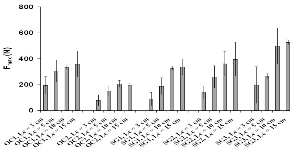
Figure 3. Maximum pull-out strength measurement in function of embedded length.
