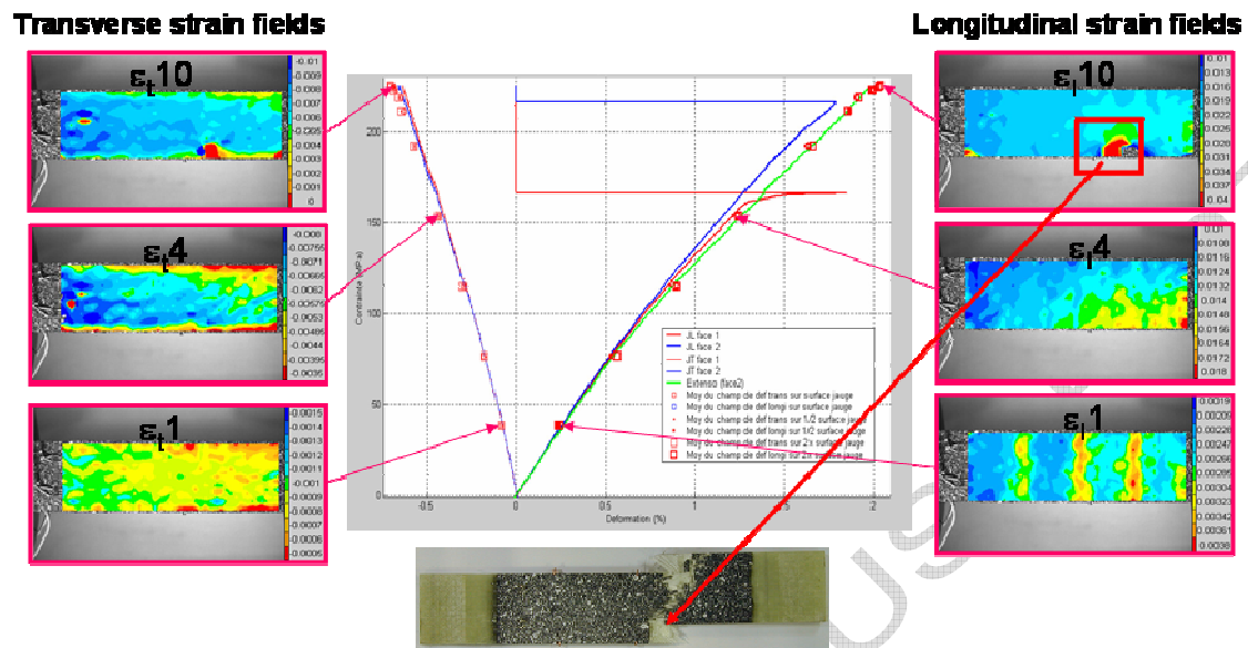
Figure 13 : Multi-instrumentation results, 10 mm gauges
