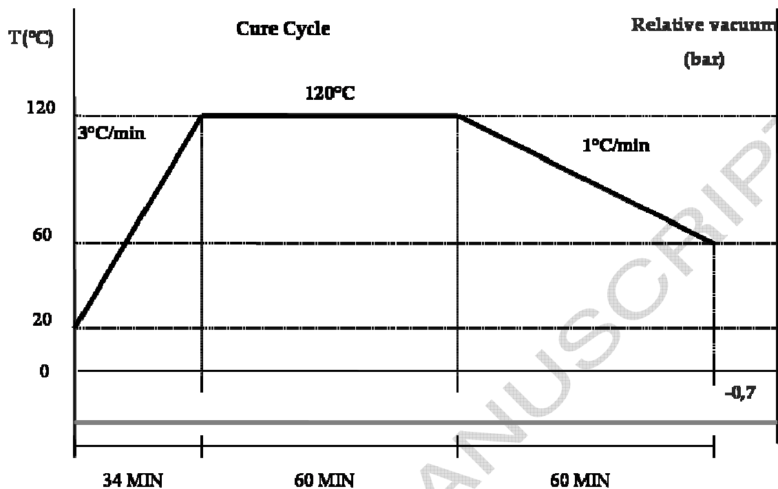
Figure 3: Cure cycle
