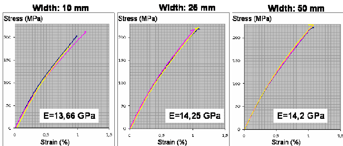
Figure 11 : Load-extension diagrams for widths: 10, 25 and 50 mm
