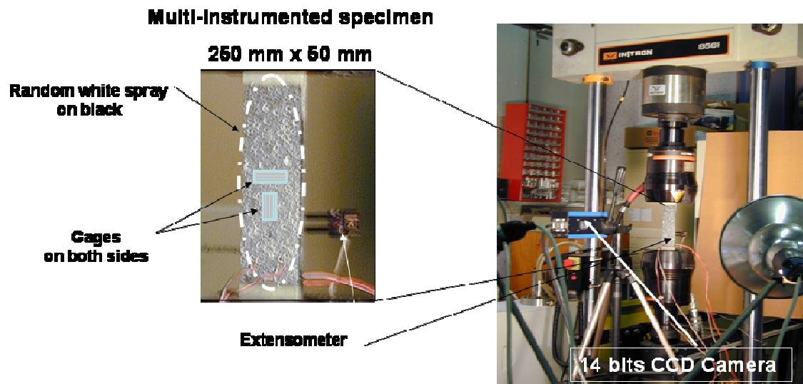
Figure 12 : Multi-instrumented specimens
