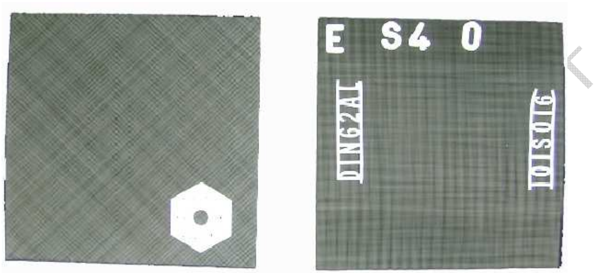
Figure 9: X radiography of test blocks (4 plies): resp. \pm 45 and 2x2 twill
