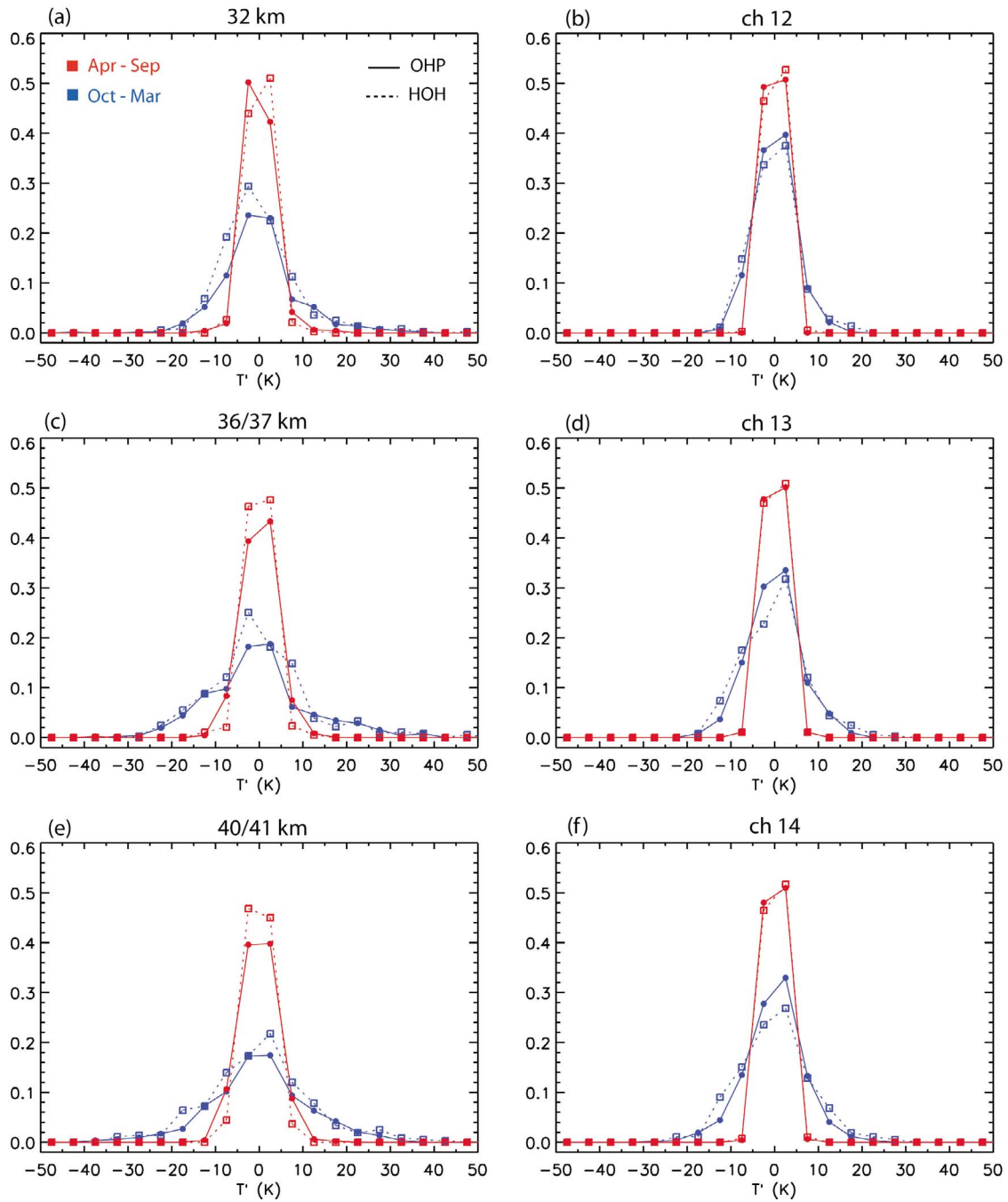
Figure 8. Summer and winter distributions of temperature anomalies of (a, c, e) lidar and (b, d, f) AMSU for OHP (solid) and HOH (dotted) stations.
