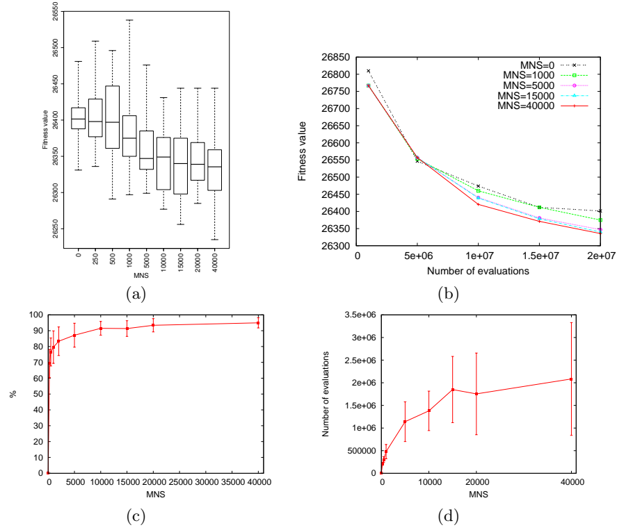
Fig. 2. Results for N=500 and M=20 . Boxplots of fitness values of the 30 solutions found after 2 \cdot 10^7 evaluations (a). Median performance according to the number of evaluations (b). Average percentage (and standard deviation) of visited local optima plateaus where the perturbation led to a portal (c). Number of evaluations (average number and standard deviation) lost during the perturbation step according to the MNS values (d).
