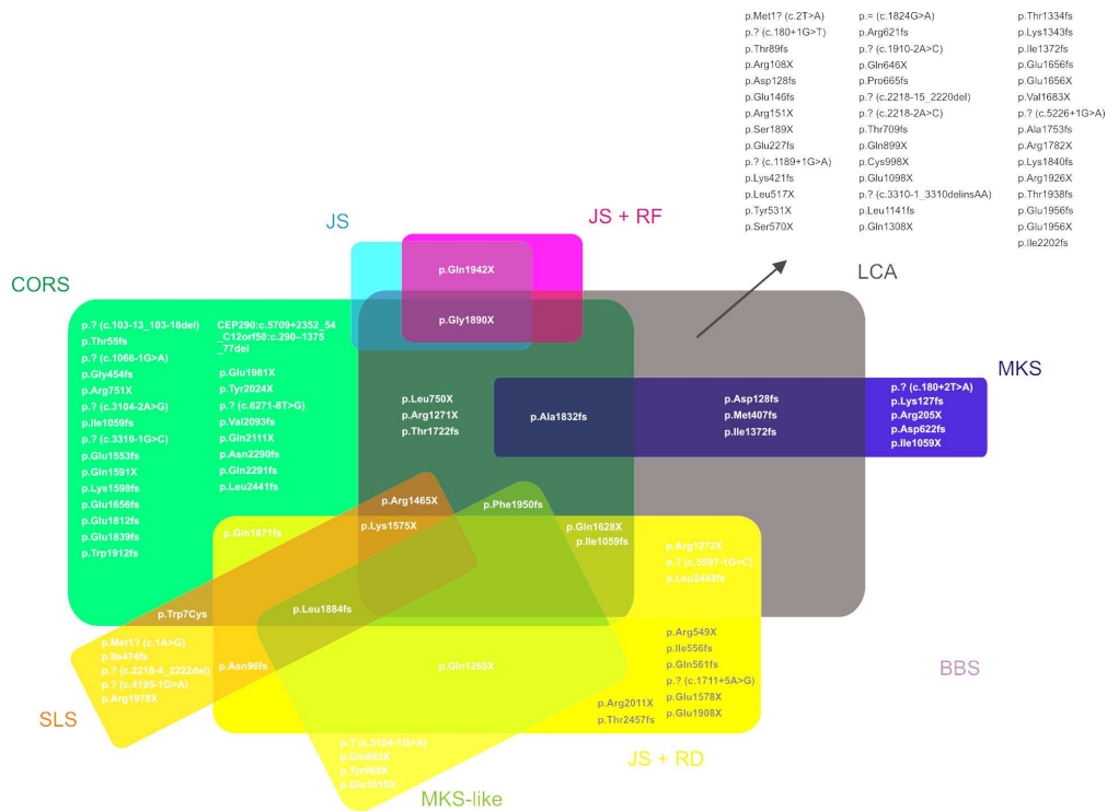
Figure 2: Overlap of CEP290 mutations between different diseases.
