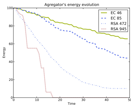
Figure 2. Comparison of energy consumption
