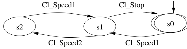
Fig. 5. The transition system TS_o corresponding to the interface OIManual
