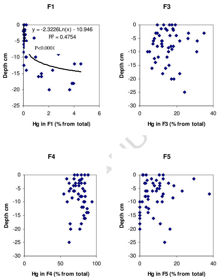
Fig. 7: Vertical distribution of relative Hg content (%) in each fraction, at the polluted stations.
